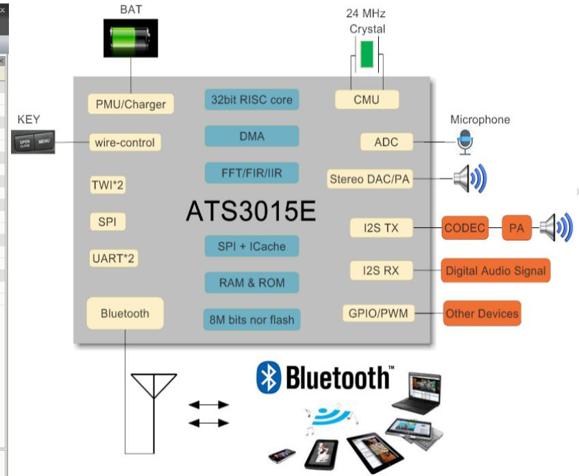
Figure 1-1 ATS3015E Application Diagram
